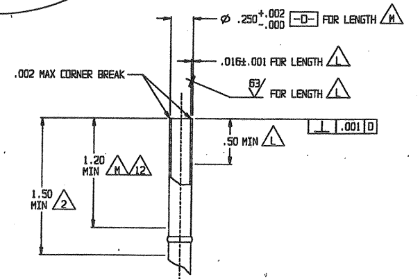
VIEW E FOR -1 AND -101 SCALE 2/1
