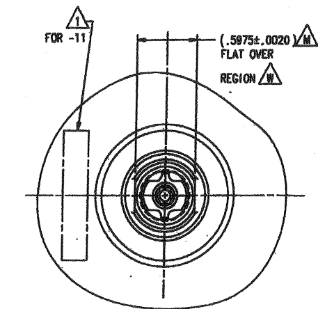
VIEW J-J SCALE: 2/1
