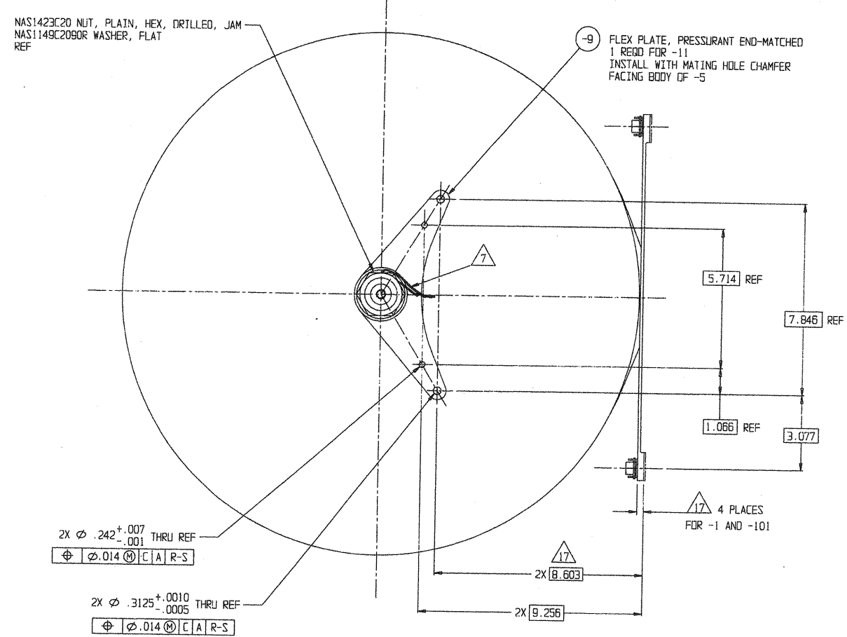
VIEW Y-Y SHEET 1
