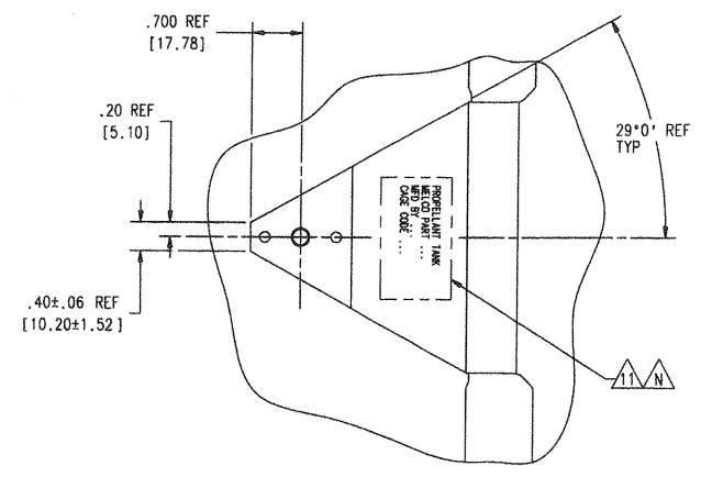
VIEW U SHEET 1
