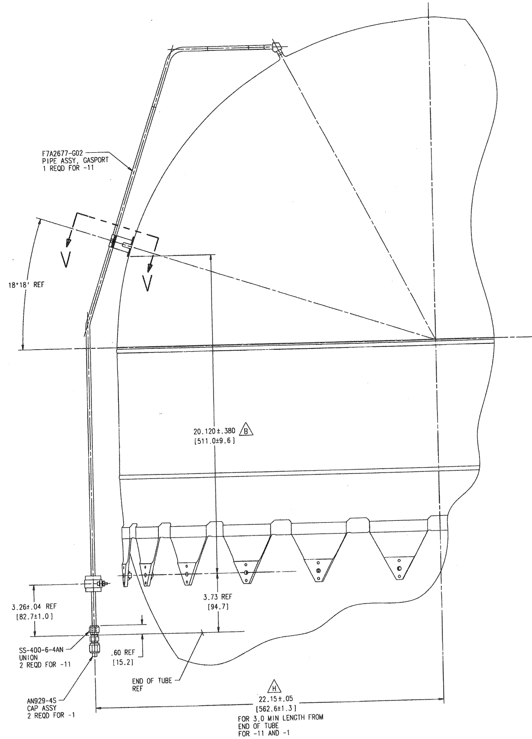
VIEW K-K SHEET 1 ROTATED 7°30' COUNTERCLOCKWISE SCALE: 1/2
