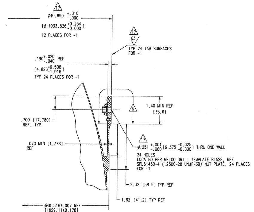
SECTION J-J SHEET 1 BACKGROUND GEOMETRY OMITTED FOR CLARITY
