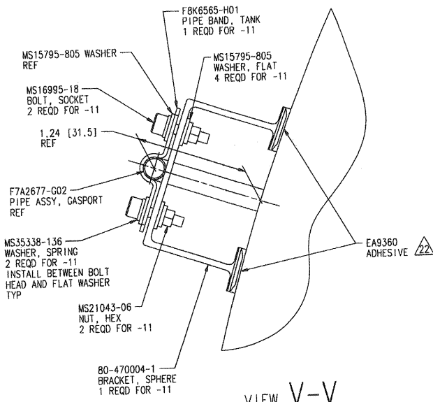
VIEW V-V PARTIAL BACKGROUND OMITTED FOR CLARITY SCALE: 2/1
