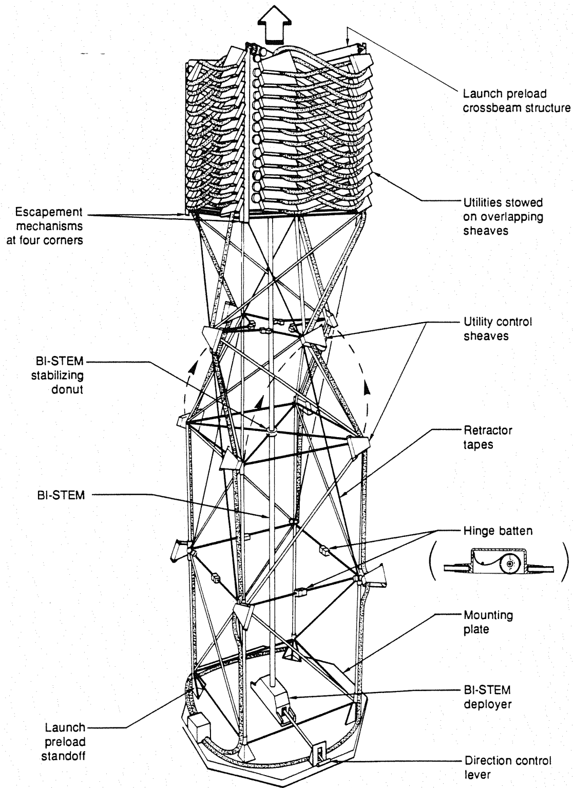
Figure 1. Space Station deployable boom.
