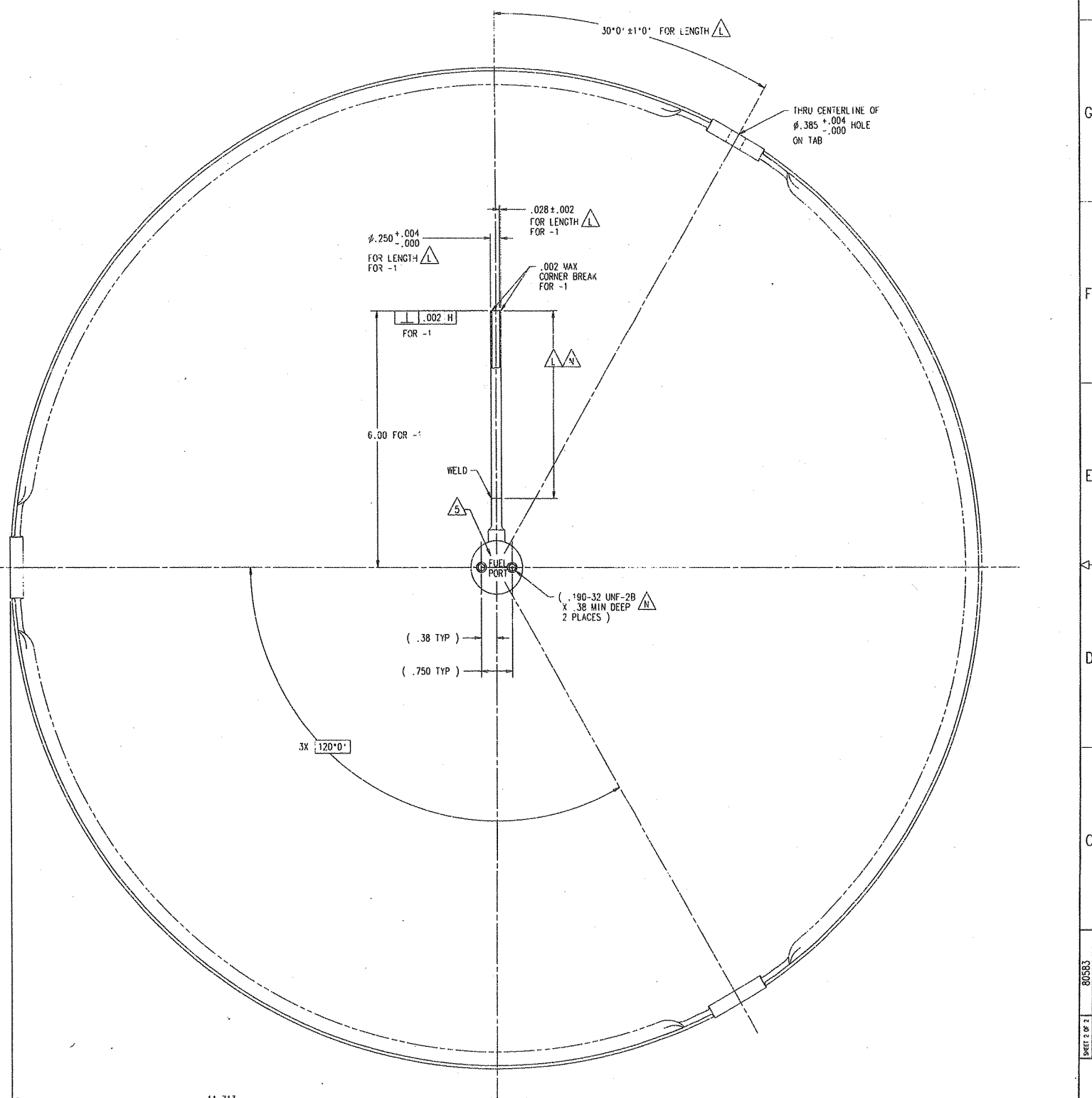
VIEW X-X SHEET 1
