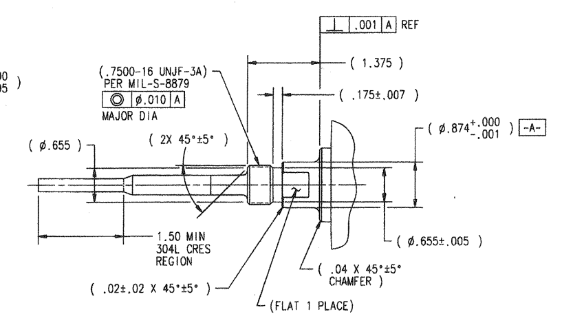
VIEW A FOR -1
