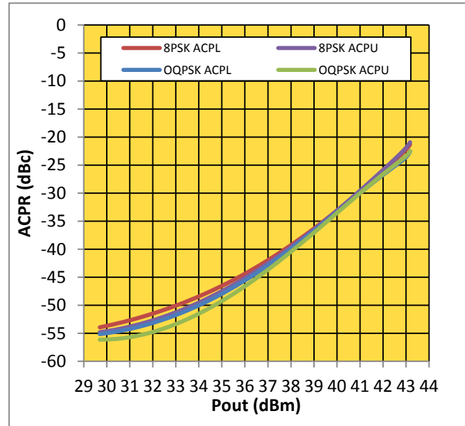
OQPSK ACPR -25 dBc @ 30GHz CW in Fixture *
