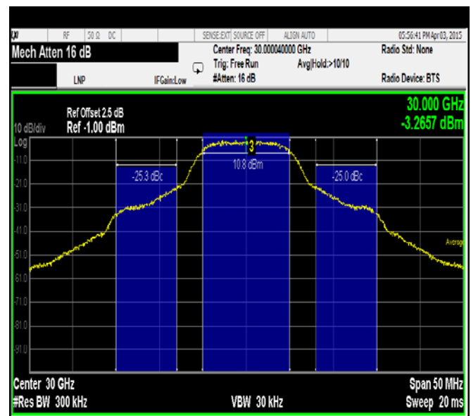
OQPSK ACPR -25 dBc @ 30GHz CW in Fixture *
