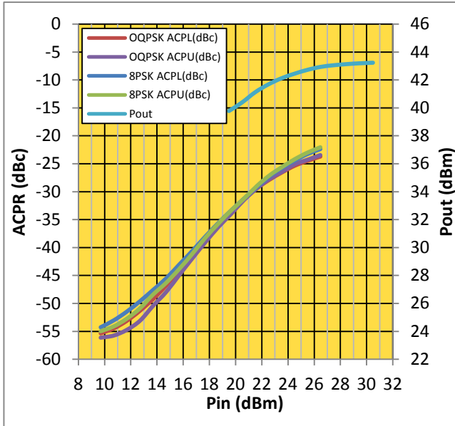
8PSK ACPR -25 dBc @ 30GHz CW in Fixture *
