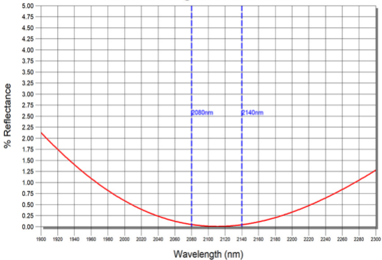
A1505: MAXCOAT AR @ 2080 - 2140nm on CTH:YAG
